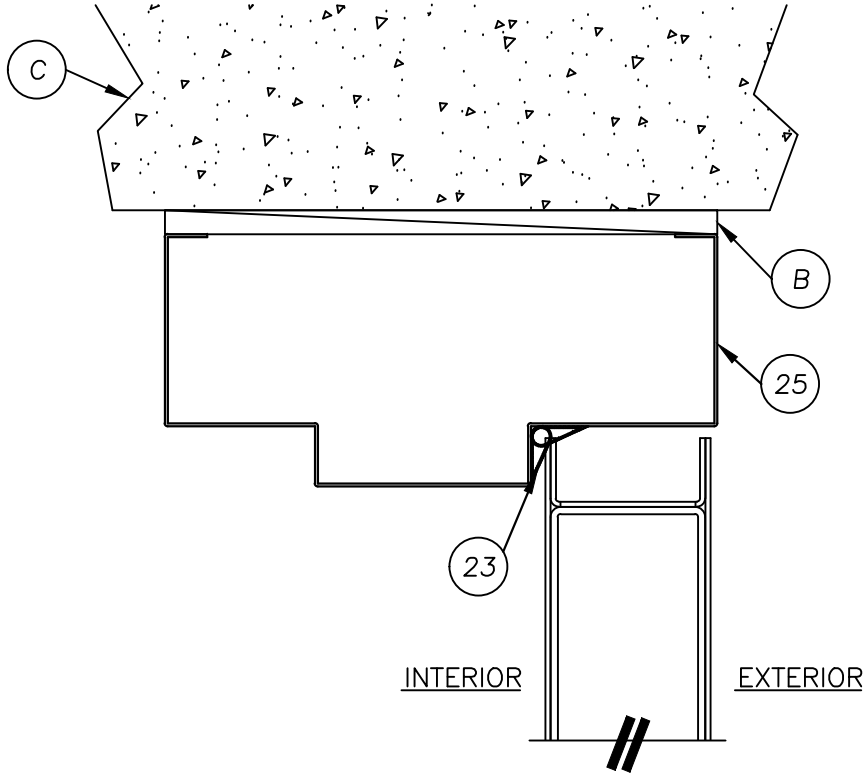
1 6 VERTICAL CROSS SECTION @ HEAD
