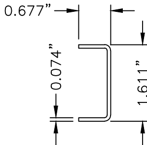
1 DOOR STILE EDGE REINFORCEMENT
