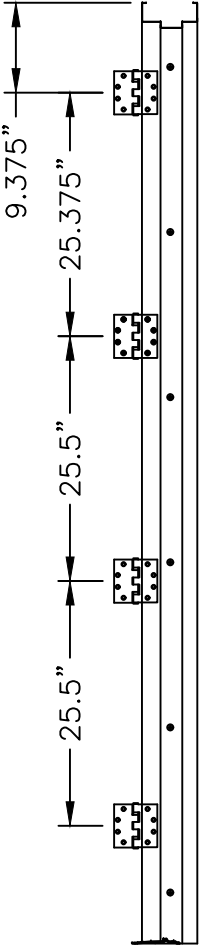
HINGE LOCATIONS 2" HEAD
